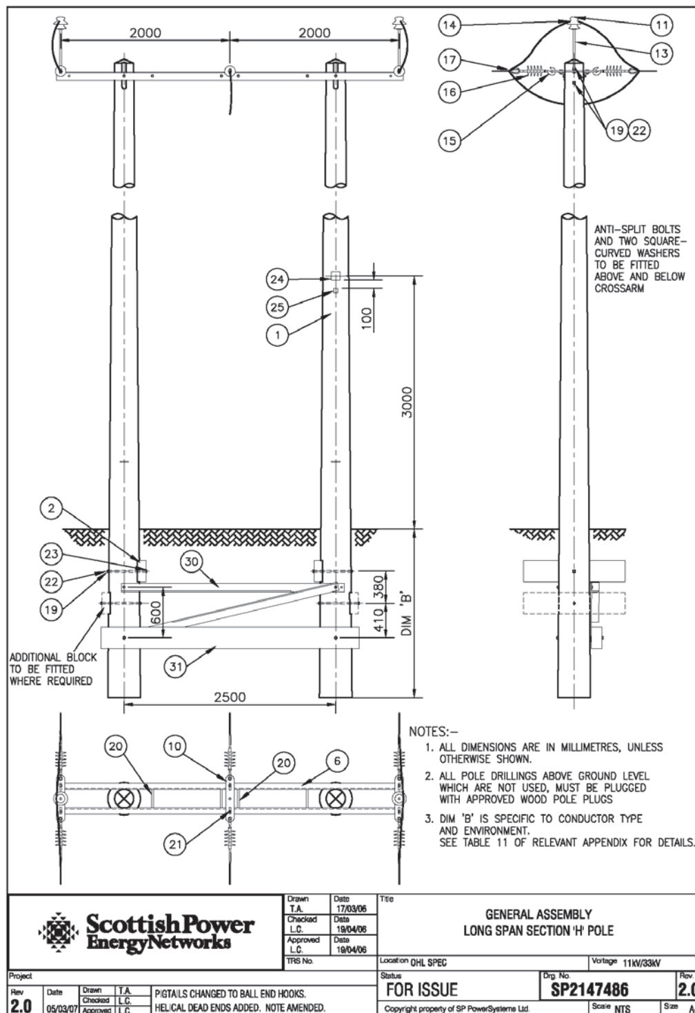
Figure 14 Long Span "H" Pole Straight Line or Angle Section (Drawing SP2147486)
